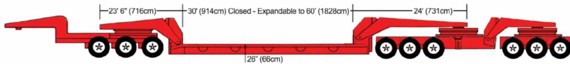
9 & 13 Axle Schnable with Steerable Dolly
